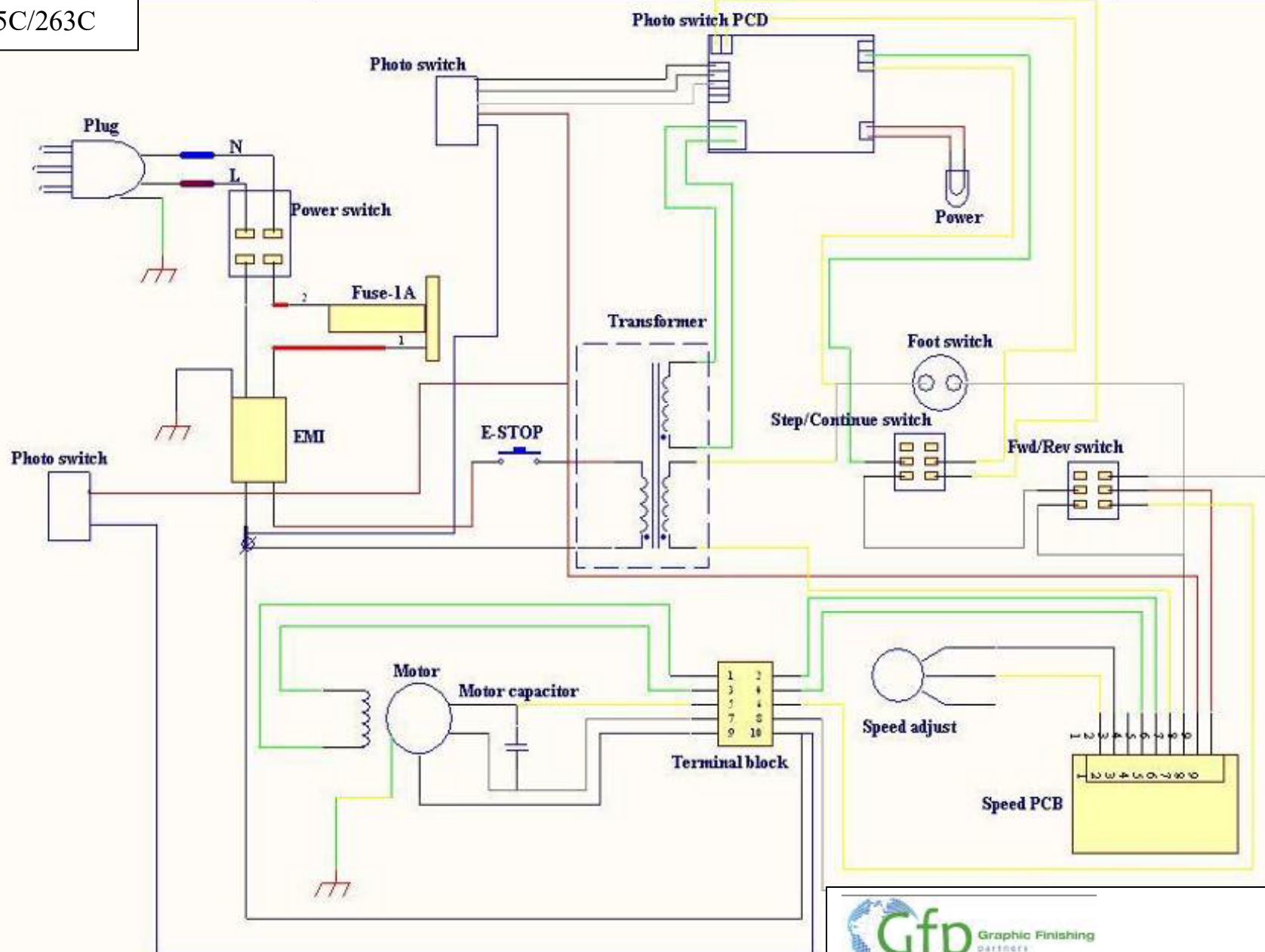
View 6 – Wiring Diagram
