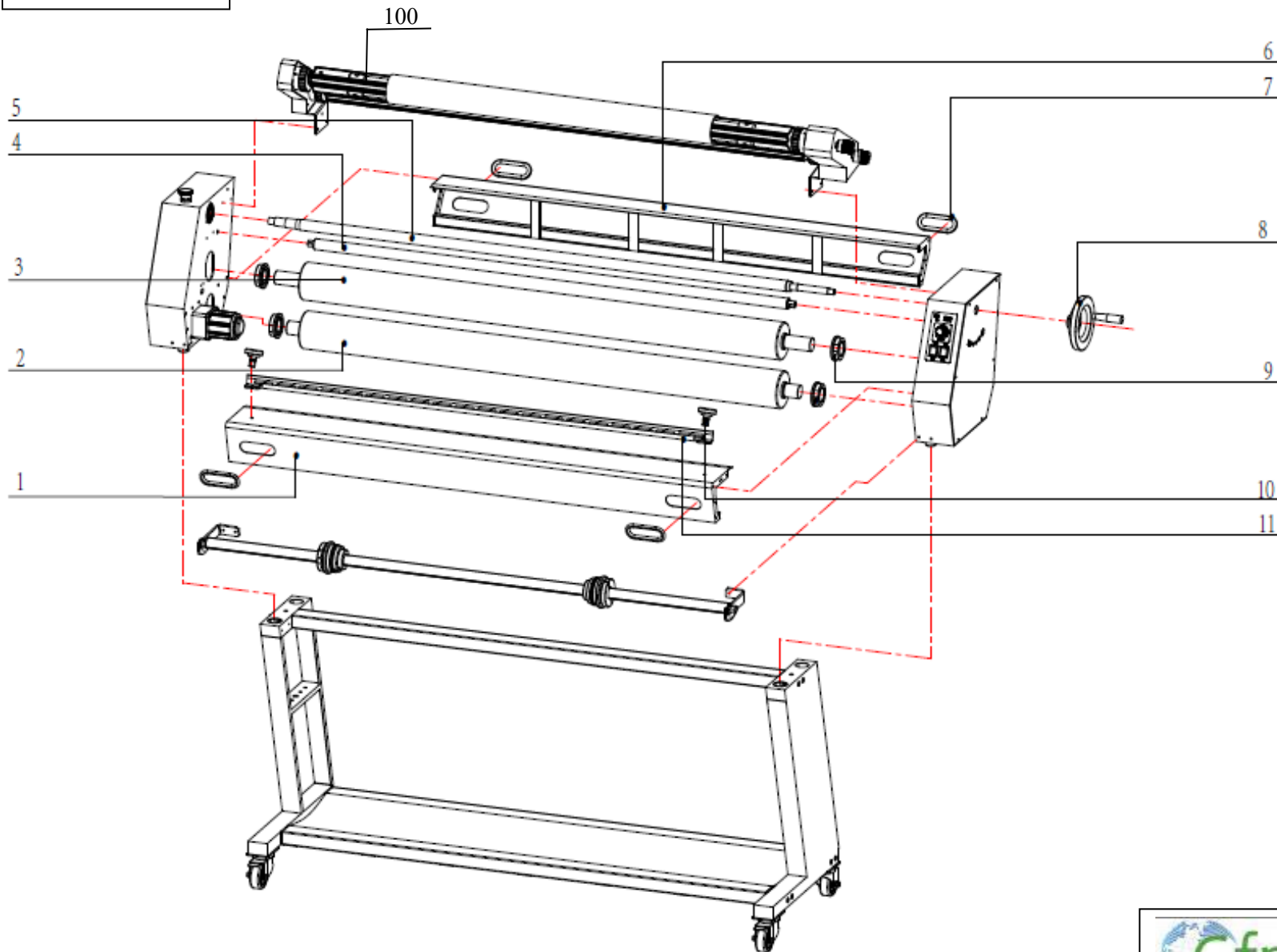
View 1- Frame and Stand
